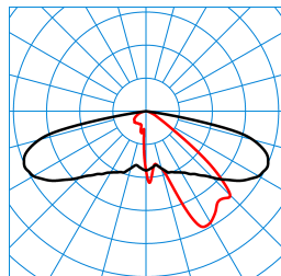
Publisca P1-AB2L-LRA/2000-730 3G1S ET (CLO end value) TX301117 DIN 5040: A30 UTE: 1,00 l CEN Flux Code: 34 71 96 100 100
