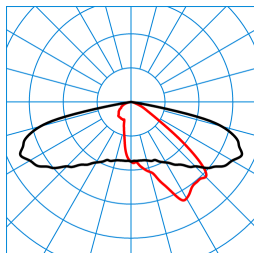
LIQ 50N-AB2L-LRA/3200-740 4G1 ETDD (CLO initial value) TX278270
