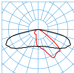
LIQ 50N-AB2L-LR/220/260/320-727 4G1 ET (CLO initial value) TX277999
