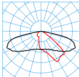
LIQ 50N-AB2L-LR/1350-727 2G1 ET (CLO initial value) TX277879
