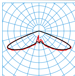
Publisca P1W-RB6L-LRA/2200-740 3G1S TX053546 DIN 5040: A20 UTE: 1,00 J CEN Flux Code: 19 57 99 100 100 0 50 50 0
