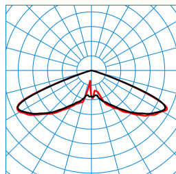
Publisca P1W-RB6L-LRA/2200-740 3G1S ET (CLO initial value) TX301207 DIN 5040: A20 UTE: 1,00 J CEN Flux Code: 19 57 99 100 100 0 50 50 0
