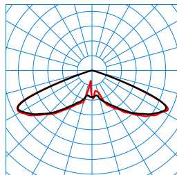
Publisca P1W-RB6L-LRA/2200-740 3G1S ET (CLO end value) TX301029 DIN 5040: A20 UTE: 1,00 J CEN Flux Code: 19 57 99 100 100 0 50 50 0
