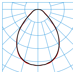
ArmoFit Act M48 PW19 53-8 ETDD8 TWW + ArmoFit Sky M48-TS ZER (ActDWW) TX426313
