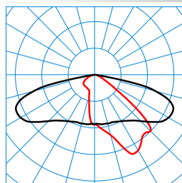
9701SG-AB2L/15/26/38-740 4G2 (1500 lm) TX064195 DIN 5040: A30 UTE: 1,00 G CEN Flux Code: 35 71 96 100 100
