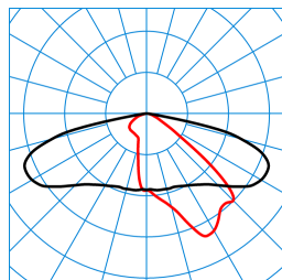
9701SG-AB2L/15/26/38-740 4G2 (3800 lm) TX064197 DIN 5040: A30 UTE: 1,00 G CEN Flux Code: 35 71 96 100 100
