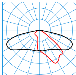
9701SG-AB2L/15/26/38-740 4G2 (2600 lm) TX064196 DIN 5040: A30 UTE: 1,00 G CEN Flux Code: 35 71 96 100 100
