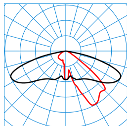
Publisca P2-AB2L-LRA/5100-730 6G1S ET (CLO initial value) TX300472 DIN 5040: A30 UTE: 1,00 G CEN Flux Code: 35 74 97 100 100
