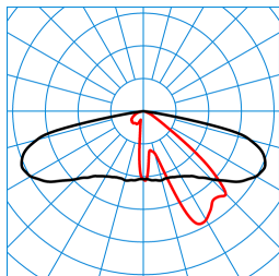
Publisca P2-AB2L/1500-740 2G1S ETDD (CLO end value) TX300418
