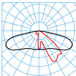
Publisca P2-AB2L/1500-740 2G1S ETDD (CLO initial value) TX301133
