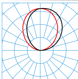
Sanesca W2 LED2600-830 03 TX371869
