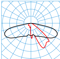
Publisca P2-AB2L-LRA/2600-730 3G1S ET (CLO end value) TX300695 ■ C0 - C180 ■ C90 - C270 DIN 5040: A30 UTE: 1,00 l CEN Flux Code: 34 71 96 100 100
