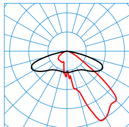
Publisca P2-AB2L-LR/2900-740 4G1S ET (CLO end value) TX300256 DIN 5040: A30 UTE: 1,00 G CEN Flux Code: 35 73 97 100 100
