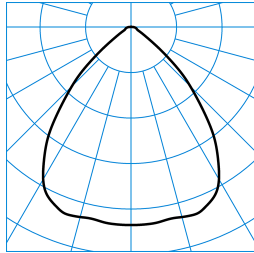
InperiaL G2 C07 HR22 2700-830 03 + ZN-PC ■ C0 - C180 TX373418
