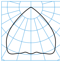
InperiaL G2 C07 HR22 2700-830 03 ■ C0 - C180 TX373429
