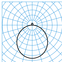
Solegra WD1 OTA 2600-830 + WD1 ZP 03 TX374258
