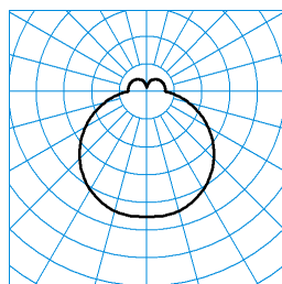
Solegra WD1 OTA 2600-830 + WD1 ZPF-T C1/C TX374896
