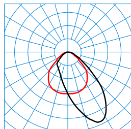
LuceoS D/H2-L CDP-A 5000-840 ETDD 03 (Pendant ZS/ZST+EB3) TX245968 DIN 5040: A50 UTE: 1,00 D CEN Flux Code: 60 88 97 100 100 0 0 0 0
