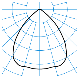
InperiaL G2 C07 BR22 2700-830 01 + ZN-PC TX373501 ■ C0 - C180
