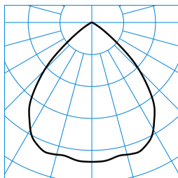
InperiaL G2 C07 BR22 2700-830 01 + RD-PC TX373503 ■ C0 - C180
