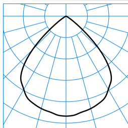
InperiaL G2 C07 BR22 2700-830 01 TX373505 ■ C0 - C180
