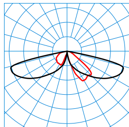
CS 19 100-AB2L-LR/1200-730 2G1S ET (CLO initial value) TX299977 DIN 5040: A20 UTE: 1,00 l CEN Flux Code: 26 63 96 100 100
