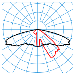
Publisca P1W-AB2L-LRA/1200-740 2G1S TX053492 DIN 5040: A30 UTE: 1,00 l CEN Flux Code: 32 69 96 99 100 0 17 50 1
