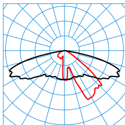
Publisca P1W-AB2L-LRA/1200-740 2G1S ET (CLO initial value) TX301134 DIN 5040: A30 UTE: 1,00 l CEN Flux Code: 32 69 96 99 100 0 17 50 1
