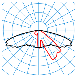
Publisca P1W-AB2L-LRA/1200-740 2G1S ET (CLO end value) TX300680 DIN 5040: A30 UTE: 1,00 l CEN Flux Code: 32 69 96 99 100 0 17 50 1
