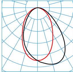
ArmoFit G2 Act M59 D-WW 53-8 ETDD8 (ActDCW) TX376367 DIN 5040: A50 UTE: 1,00 C CEN Flux Code: 61 87 98 100 100 0 0 0 0 ■ C0 - C180 ■ C90 - C270
