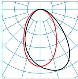
ArmoFit G2 Act M59 D-WW 53-8 ETDD8 (ActDWW) TX376403 DIN 5040: A50 UTE: 1,00 C CEN Flux Code: 61 87 98 100 100 0 0 0 0 ■ C0 - C180 ■ C90 - C270
