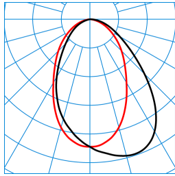
ArmoFit G2 Act M59 D-WW 53-8 ETDD8 (ActDSU) TX376462 DIN 5040: A50 UTE: 1,00 C CEN Flux Code: 61 87 98 100 100 0 0 0 0 ■ C0 - C180 ■ C90 - C270
