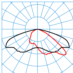
LIQ 70N-AB7L-LRA/10/12/13-722 12G1 ETDD (CLO initial value) TX280996
