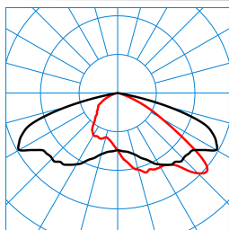
LIQ 70N-AB7L-LRA/10/12/13-722 12G1 ETDD (CLO end value) TX280895
