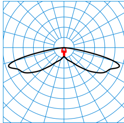
Publisca P2-SB3L/1200-730 2G1S ETDD (CLO end value) TX300796
