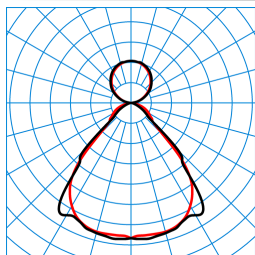
SFlow H3-L MRW LED6400-840 LLWS 03 TX053188
