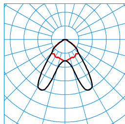
E-Line Fi LightP DA-B-DA 80-840 L75 01 (150) TX372552
