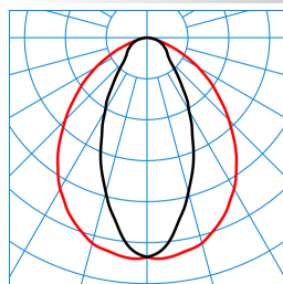
Nextrema G3 TB 60-840 +LV TWP PC TX374481
