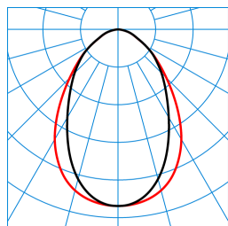
ArimoFit Act M46 DW19 42-8 ETDD8 + ArimoFit Sky M46-TS ZER (ActDSU) TX426268
