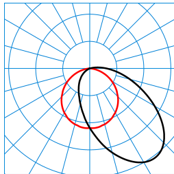
Sanesca W3-S2/R LED5000-840 01 (reading light) TX05794
