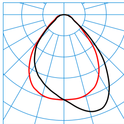
ArimoFit G2 Act M59 P-WW 53-8 ETDD8 (ActDWW) TX376408 ■ C0 - C180 ■ C90 - C270 DIN 5040: A50 UTE: 1,00 C CEN Flux Code: 66 90 97 100 100
