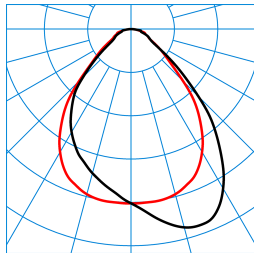
ArimoFit G2 Act M59 P-WW 53-8 ETDD8 (ActDCW) TX376493 ■ C0 - C180 ■ C90 - C270 DIN 5040: A50 UTE: 1,00 C CEN Flux Code: 66 90 97 100 100
