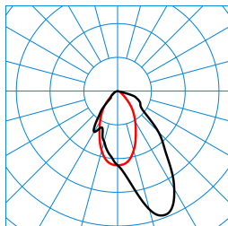
CreavoAct M57 LWW-03 42-8 ETDD8 01(CTDCW) TX195459 ■ C0 - C180 ■ C90 - C270 DIN 5040: A50 UTE: 1,00 C CEN Flux Code: 70 92 99 100 100
