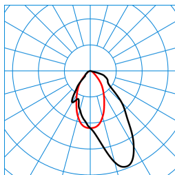
CreavoAct M57 LWW-03 42-8 ETDD8 01(CTDSU) TX195460 ■ C0 - C180 ■ C90 - C270 DIN 5040: A50 UTE: 1,00 C CEN Flux Code: 70 92 99 100 100
