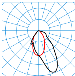
CreavoAct M57 LWW-03 42-8 ETDD8 01(CTDWW) TX195461 ■ C0 - C180 ■ C90 - C270 DIN 5040: A50 UTE: 1,00 C CEN Flux Code: 70 92 99 100 100
