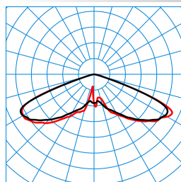
Publisca P2-RB6L-LRA/2600-740 3G1S TX047900 ■ C0 - C180 ■ C90 - C270 DIN 5040: A20 UTE: 1,00 J CEN Flux Code: 20 57 98 100 100
