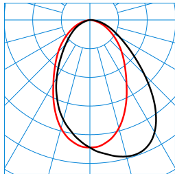
ArimoFit G2 Act M57 D-WW 42-8 ETDD8 (ActDCW) TX376383 DIN 5040: A50 UTE: 1,00 C CEN Flux Code: 61 87 98 100 100 0 0 0 0 ■ C0 - C180 ■ C90 - C270
