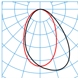
ArimoFit G2 Act M57 D-WW 42-8 ETDD8 (ActDWW) TX376390 DIN 5040: A50 UTE: 1,00 C CEN Flux Code: 61 87 98 100 100 0 0 0 0 ■ C0 - C180 ■ C90 - C270
