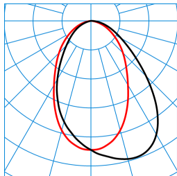
ArimoFit G2 Act M57 D-WW 42-8 ETDD8 (ActDSU) TX376396 DIN 5040: A50 UTE: 1,00 C CEN Flux Code: 61 87 98 100 100 0 0 0 0 ■ C0 - C180 ■ C90 - C270
