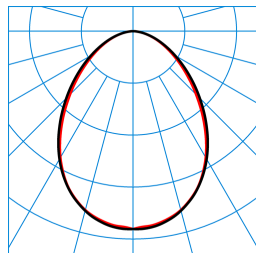
SFlow C2-L MRWD LED4000-840 01 TX050952
