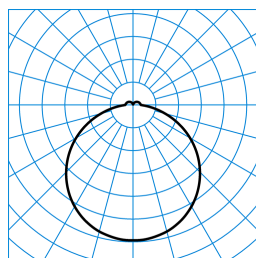
Olisq Act RWD3 DW 50 ETDD8 PC + Olisq RWD3 ZDR 1/2 03 (ActDWW) TX428598
