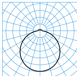
Olisq Act RWD3 DW 50 ETDD8 PC (ActDSU) TX375711
