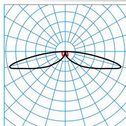
CS 19 100-SB3L/1650-740 2G1S ETDD (CLO end value) TX300149
