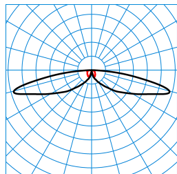
CS 19 100-SB3L/1650-740 2G1S ETDD (CLO initial value) TX300150
