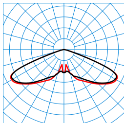
Publisca P2-RB6L/5600-740 6G1S ETDD (CLO end value) TX301509
