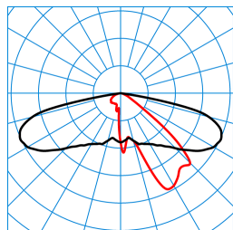
Publisca P1-AB2L-LR/2600-740 3G1S ET (CLO initial value) TX300689 DIN 5040: A30 UTE: 1,00 l CEN Flux Code: 34 71 96 100 100
