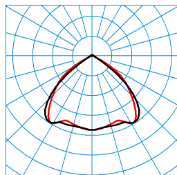
E-Line Fi LightP B-B-B 65-830 L75 03 (150) TX372529
