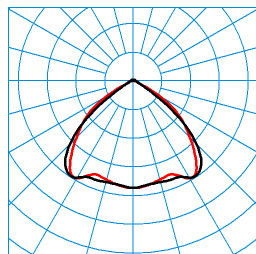
E-Line Fi LightP B-B-B 65-830 L75 03 (225) TX372142
