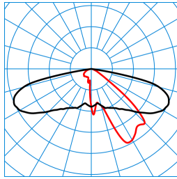
Publisca P1-AB2L-LR/2400-730 3G1S ET (CLO initial value) TX301476 DIN 5040: A30 UTE: 1,00 l CEN Flux Code: 34 71 96 100 100
