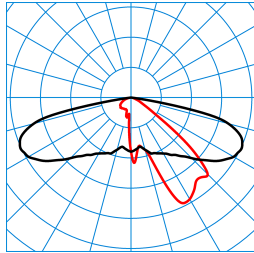
Publisca P1-AB2L-LR/2400-730 3G1S ET (CLO end value) TX301759 DIN 5040: A30 UTE: 1,00 l CEN Flux Code: 34 71 96 100 100
