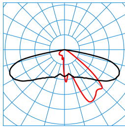
Publisca P1-AB2L-LR/2400-730 3G1S TX047521 DIN 5040: A30 UTE: 1,00 l CEN Flux Code: 34 71 96 100 100
