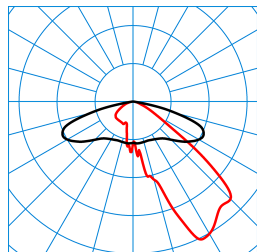
Publisca P1-AB2L-LR/3200-730 4G1S ET (CLO end value) TX300577 DIN 5040: A30 UTE: 1,00 G CEN Flux Code: 35 73 97 100 100
