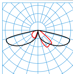
CS 19 100-AB2L-SLR1/2200-740 2G1S ET (CLO end value) TX300012 DIN 5040: A20 UTE: 1,00 l CEN Flux Code: 26 63 96 100 100
