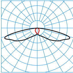
LIQ 50N-SB3L-LR-SLR2/2200-722 2G1 ET (CLO end value) TX280897
