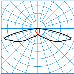
LIQ 50N-SB3L-LR-SLR2/2200-722 2G1 ET (CLO initial value) TX280990
