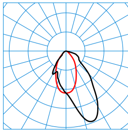
CreavoAct M57-TS LWW-03 42-8 ETDD8 01 (ACTDSU) TX195466 DIN 5040: A50 UTE: 1,00 C CEN Flux Code: 70 92 99 100 100 ■ C0 - C180 ■ C90 - C270
