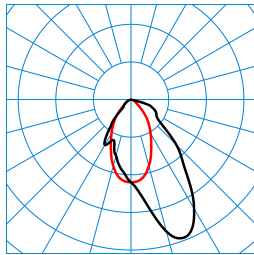
CreavoAct M57-TS LWW-03 42-8 ETDD8 01 (ACTDCW) TX195465 DIN 5040: A50 UTE: 1,00 C CEN Flux Code: 70 92 99 100 100 ■ C0 - C180 ■ C90 - C270
