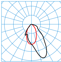
CreavoAct M57-TS LWW-03 42-8 ETDD8 01 (ACTDWW) TX195467 DIN 5040: A50 UTE: 1,00 C CEN Flux Code: 70 92 99 100 100 ■ C0 - C180 ■ C90 - C270
