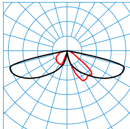
CS 19 100-AB2L-LRA/1200-730 2G1S ET (CLO initial value) TX299993
