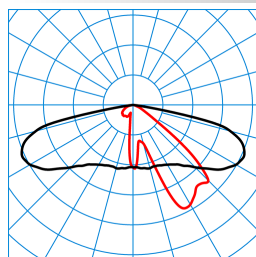
Publisca P2-AB2L-LR/1200-730 2G1S TX047735 DIN 5040: A30 UTE: 1,00 G CEN Flux Code: 34 70 96 100 100
