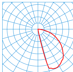
Invego Circ W1 AM16L/170-940 1G1 + IP65 24V DC 10W TX120522 ■ C0 - C180 ■ C90 - C270 DIN 5040: A30 UTE: 1,00 G CEN Flux Code: 37 73 94 100 100 0 0 0 0
