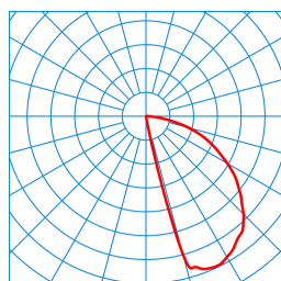
Invego Circ W1 AM16L/170-940 1G1 + IP66 24V DC 20W TX120531 ■ C0 - C180 ■ C90 - C270 DIN 5040: A30 UTE: 1,00 G CEN Flux Code: 37 73 94 100 100 0 0 0 0
