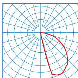
Invego Circ W1 AM16L/170-940 1G1 + IP66 24V DC 40W TX120524 ■ C0 - C180 ■ C90 - C270 DIN 5040: A30 UTE: 1,00 G CEN Flux Code: 37 73 94 100 100 0 0 0 0
