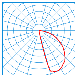
Invego Circ W1 AM16L/170-940 1G1 + IP20 24V DC 20W TX120529 ■ C0 - C180 ■ C90 - C270 DIN 5040: A30 UTE: 1,00 G CEN Flux Code: 37 73 94 100 100 0 0 0 0
