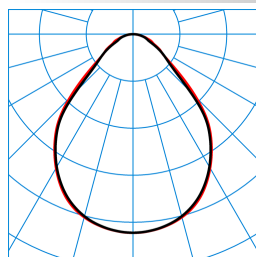
Actison Fit CDP LED12000-940 TX076392
