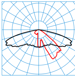
Publisca P1W-AB2L-LR/1800-740 2G1S TX053480
