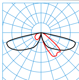
CS 19 100-AB2L-LR/5100-730 4G1S ET (CLO end value) TX300034 DIN 5040: A20 UTE: 1,00 l CEN Flux Code: 27 65 96 100 100 0 0 0 0
