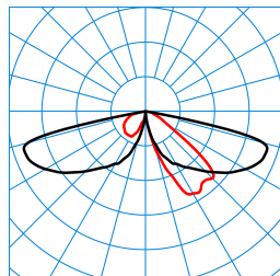
CS 19 100-AB2L-LR/5100-730 4G1S ET (CLO initial value) TX300035 DIN 5040: A20 UTE: 1,00 l CEN Flux Code: 27 65 96 100 100 0 0 0 0
