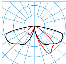
CS 19 C 100-AB2L/4200-730 4G1S ETDD (CLO initial value) TX299918
