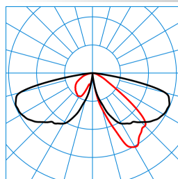
CS 19 C 100-AB2L/4200-730 4G1S ETDD (CLO end value) TX300165
