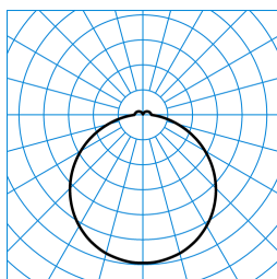
Olisq Act RWD4 DW 60 ETDD8 IP54 + Olisq RWD4 ZDR 1/2 03 (ActDWW) TX427409
