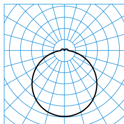
Olisq Act RWD4 DW 60 ETDD8 IP54 + Olisq RWD4 ZDR 1/2 05 (ActDWW) TX463043
