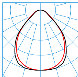
ArimoFit M73 PW19 42-840 ETDD TX149973
